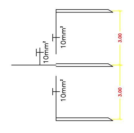
DIAGRAMA UNIFILAR
